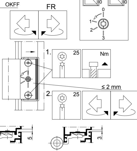
Barrel hinge for rebated doors
